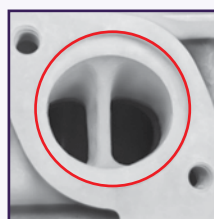
EXHAUST TWIN PORTS Centre rib Exhaust Port for better combustion
