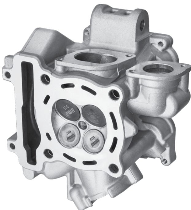
Oval Shaped Port
