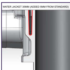
Cylinder Block Interior
